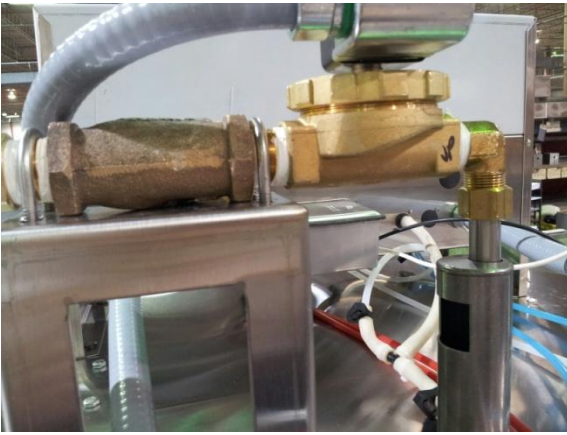
Showing the 3/4" pipe inlet, solenoid, and ASSE certified air gap.
