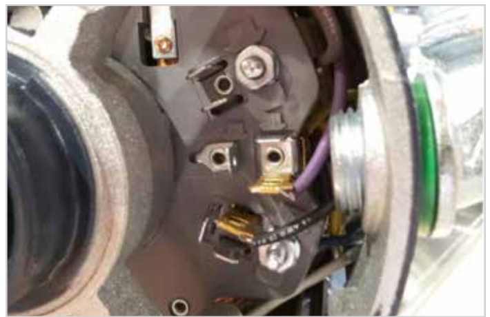
Line connection spades for L1, Neu (arrow 1 & 2)
