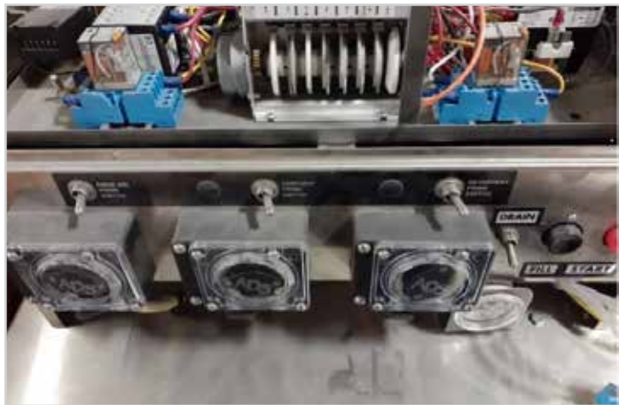
Showing AWS-H control tray in normal position
