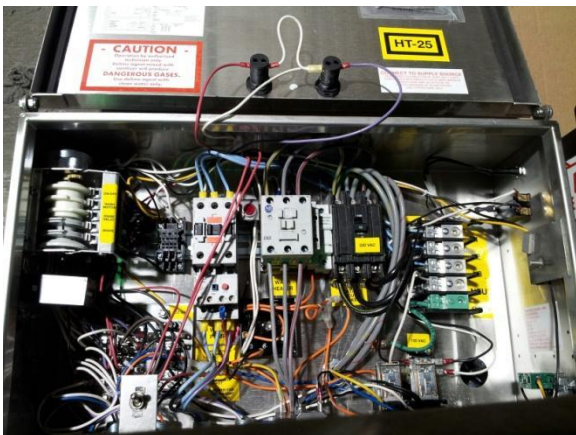
Showing HT-25, 5-wire control box
