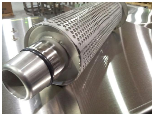
Pump filter and drain plug, note O-ring seal
