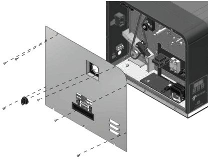
Figure 7. Accessing the cooling fan
