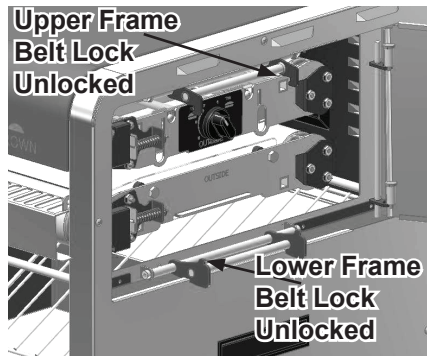
Figure 3. Conveyor locks
