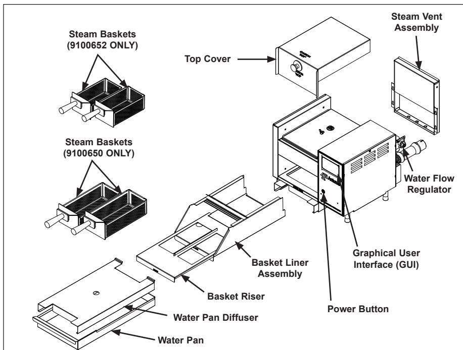
Figure 1. Components
