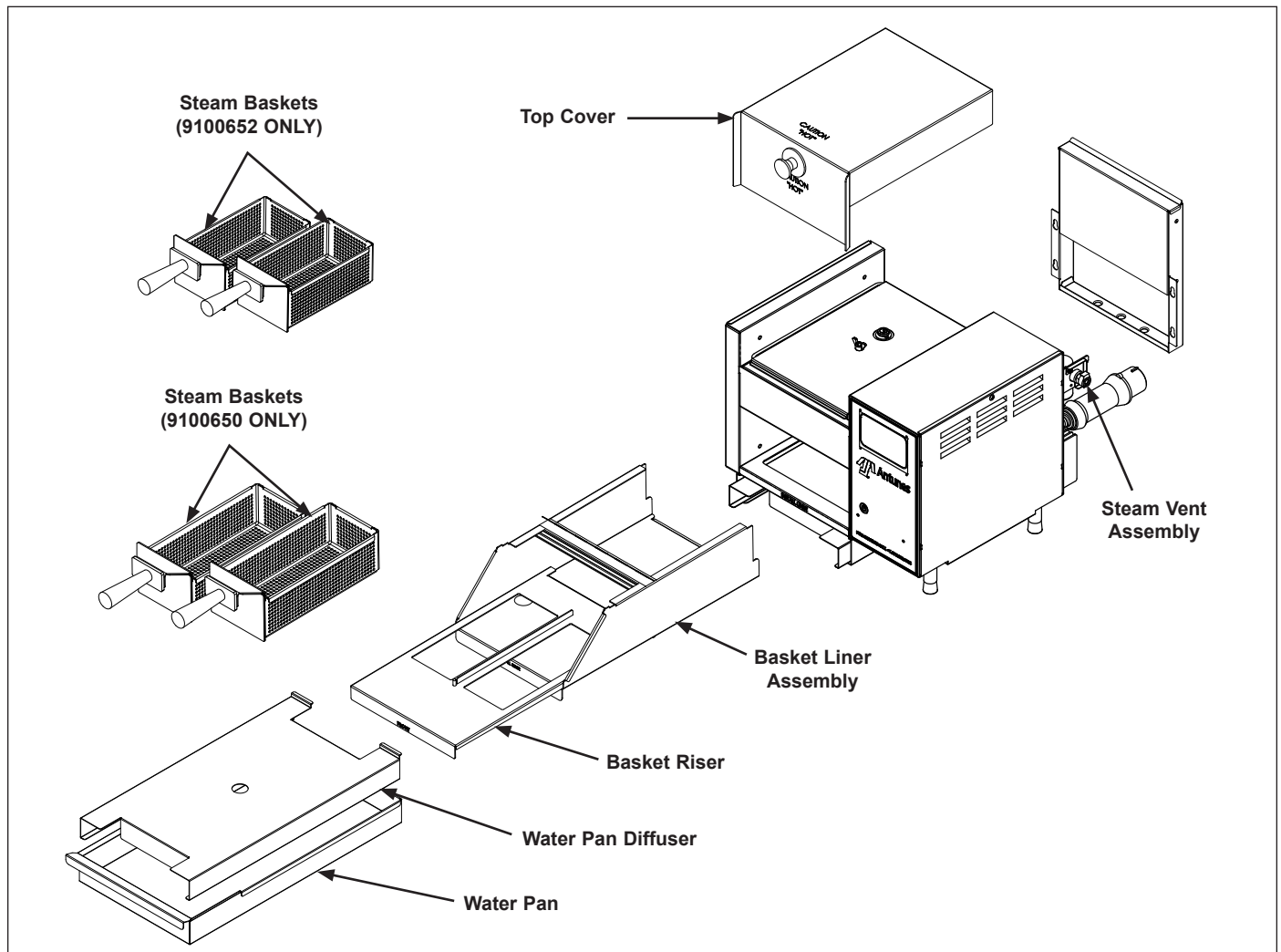
Figure 4. Components
