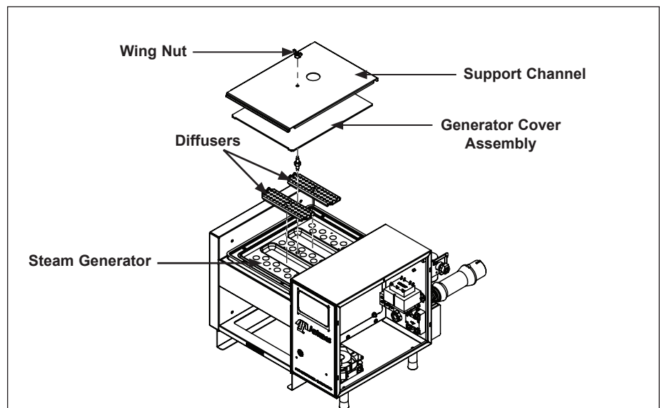
Figure 5. Steam Generator
