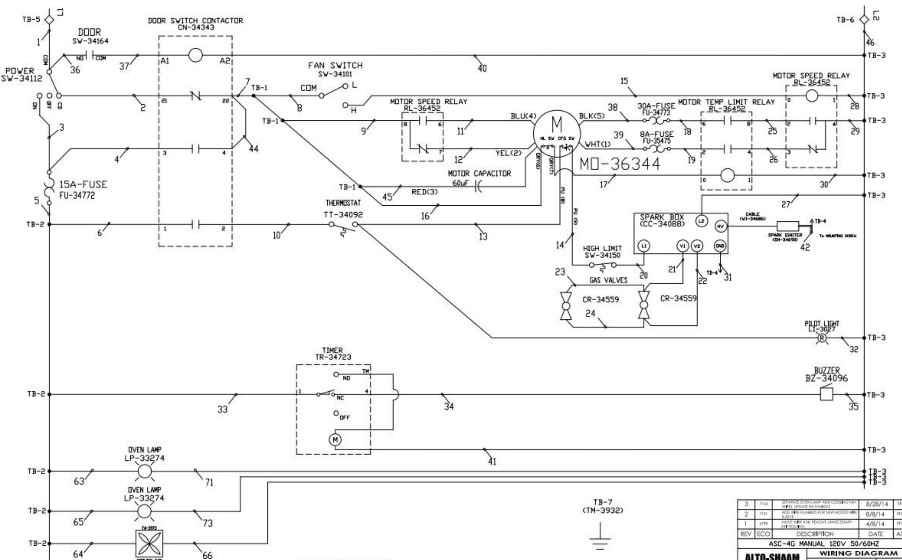
WIRE ASSEMBLY 5017050
