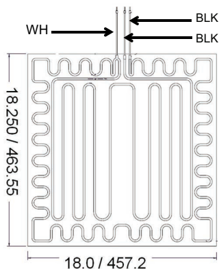
240 Volt, 750 Watts HSM-36
