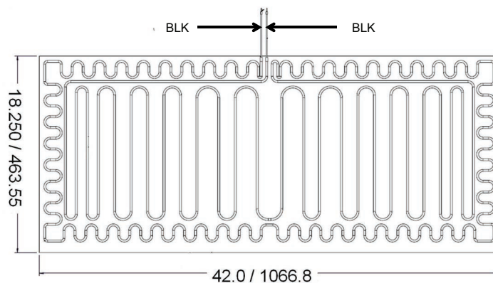
240 Volt, 1000 Watts HSM-48
