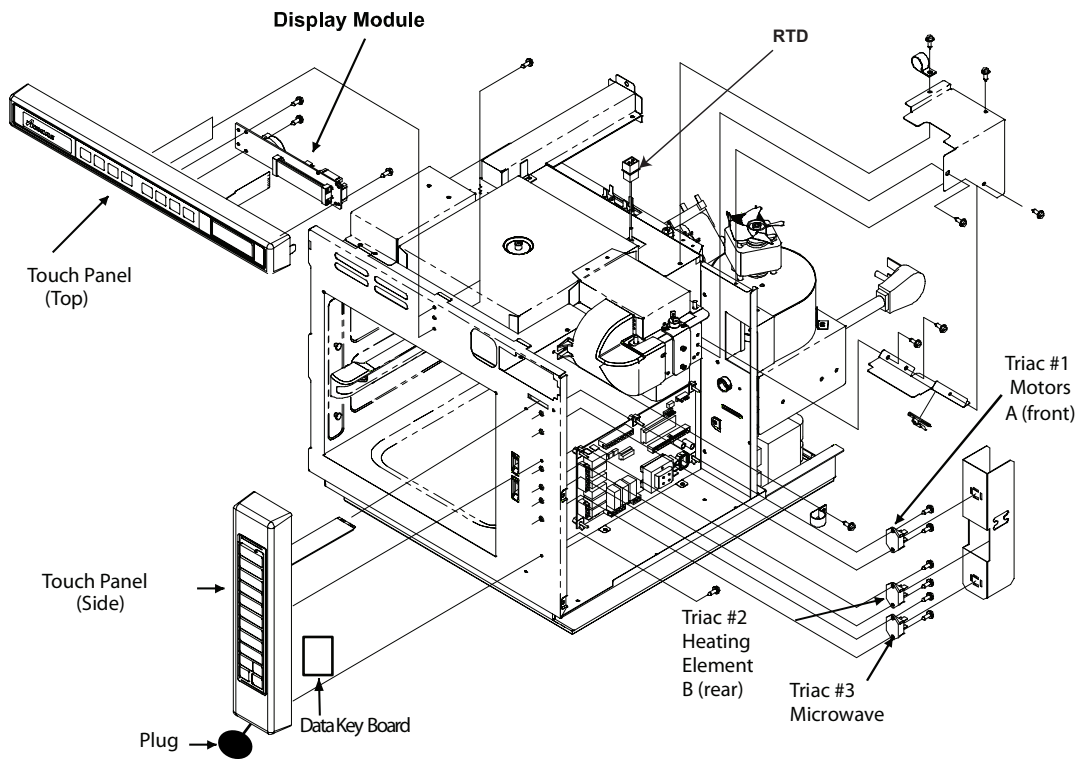
Figure 1 Touch Panels/Displays/Triacs
