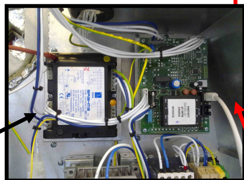
3. Combustion Control board and Blower Control board
