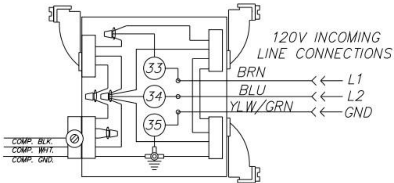
ELECTRICAL CONNECTIONS FOR MODEL 40HHC
