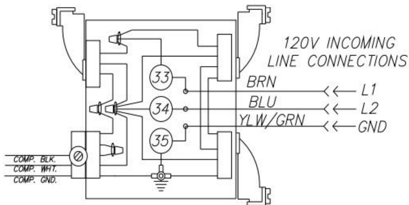
ELECTRICAL CONNECTIONS FOR MODEL 32HHC
