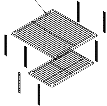
SHELF ASSEMBLY PART D
