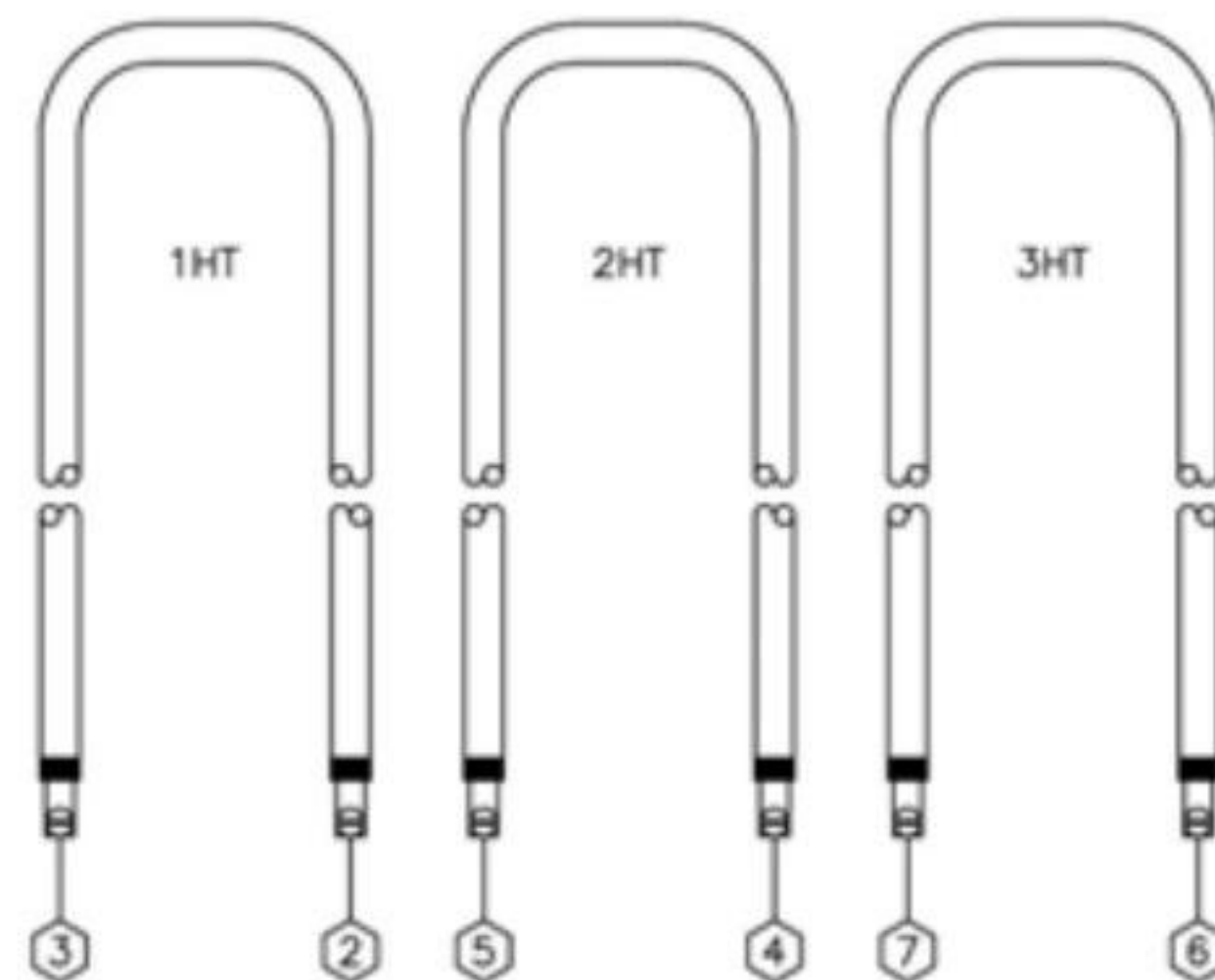
HEATER CONNECTIONS
