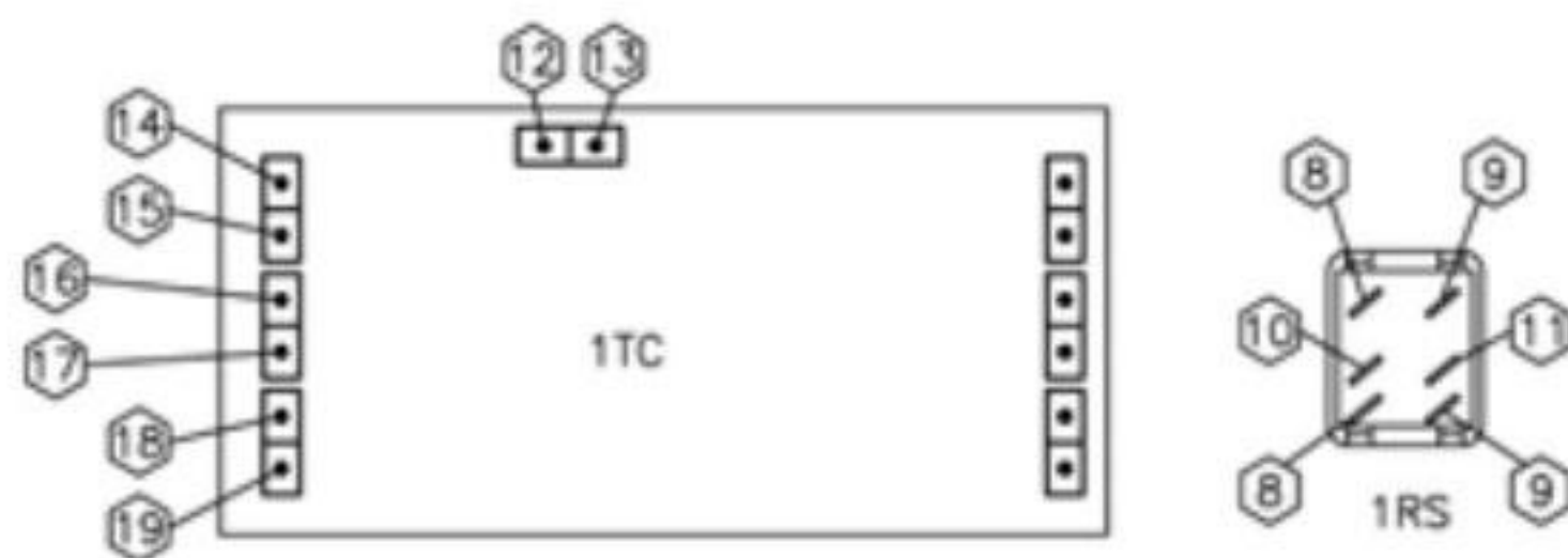
OPERATOR CONTROL PANEL (VIEWED FROM REAR WITH PANEL HINGED DOWNWARD)
