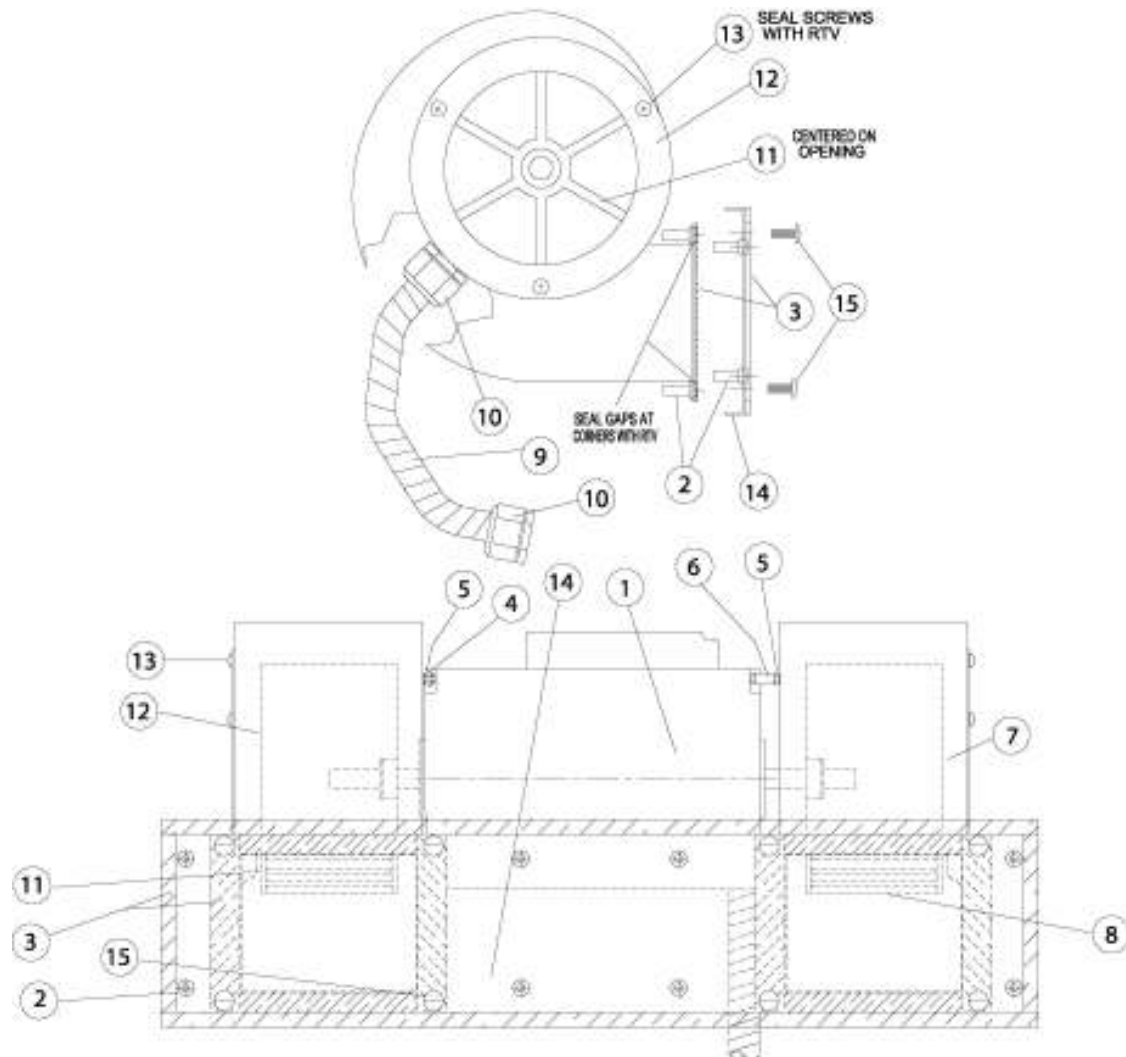
Figure 3. Blower Motor
