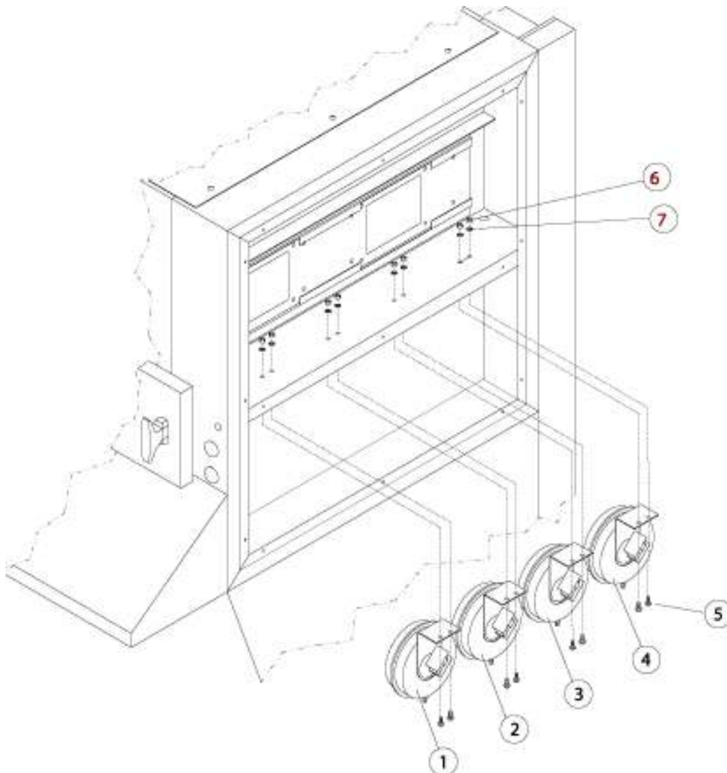
Figure 4. Right Side Cabinet
