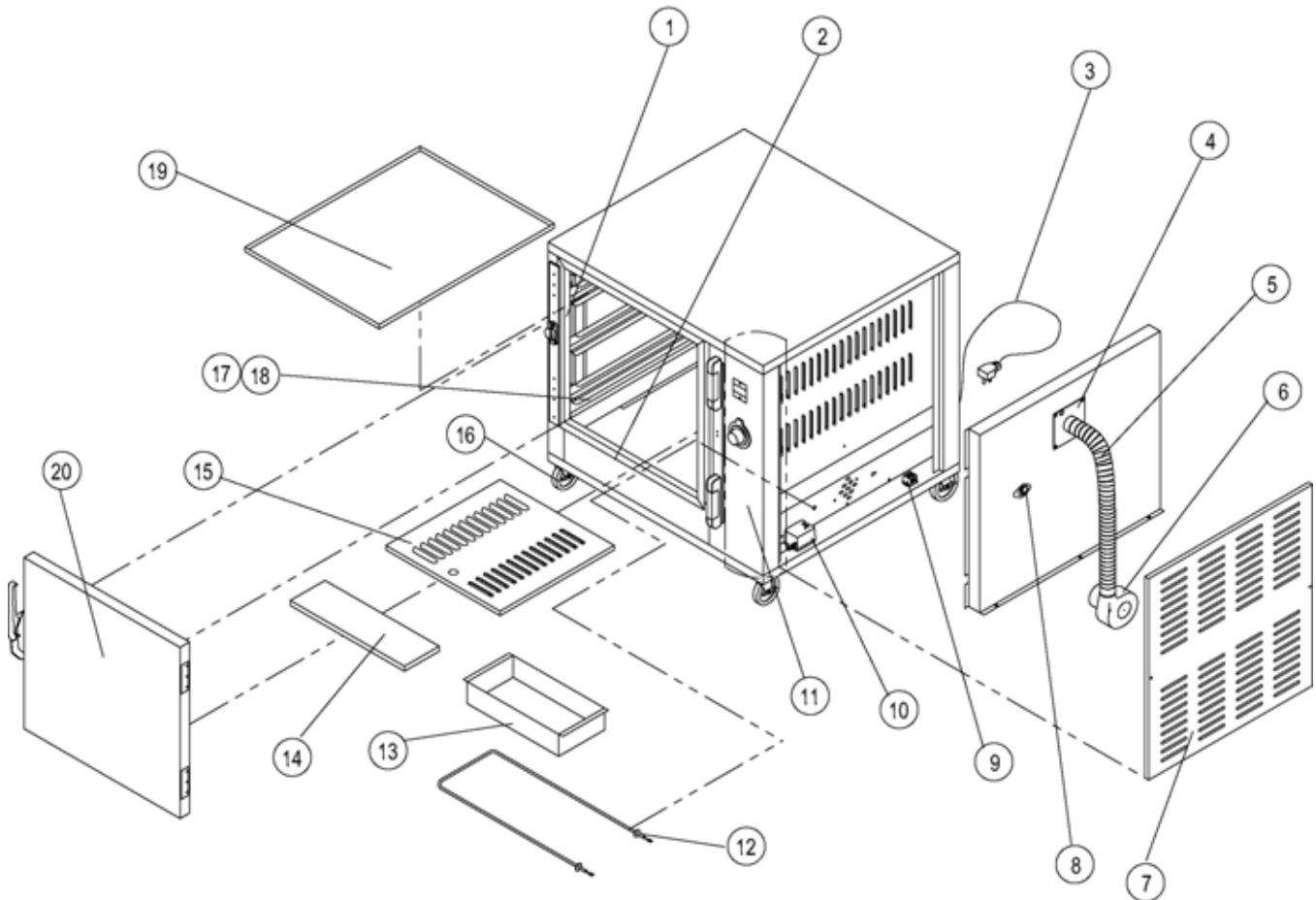
Figure 1. HHC/HHC-T Assemblies & Components
