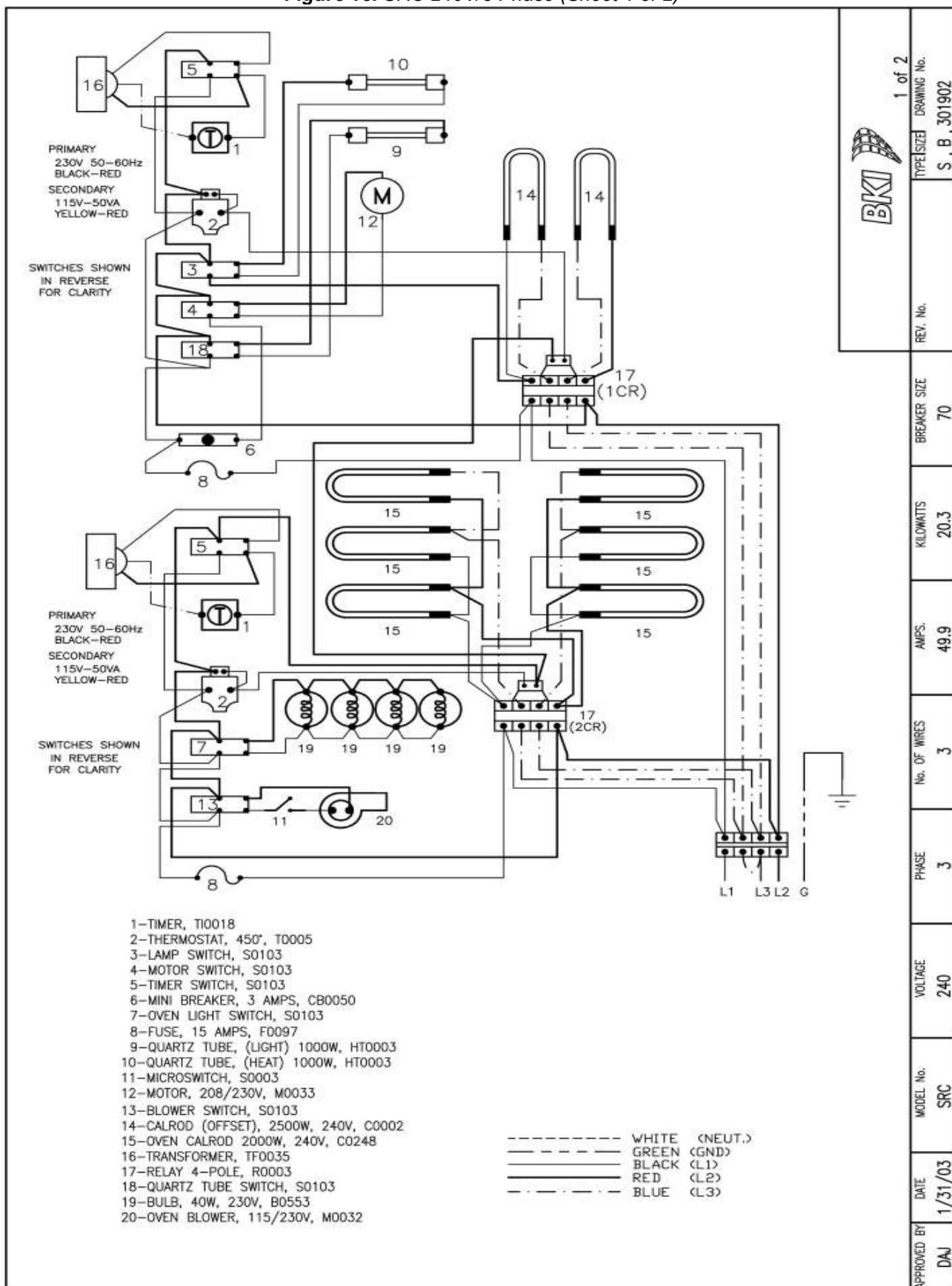
Figure 18. SRC 240V/3 Phase (Sheet 1 of 2)
