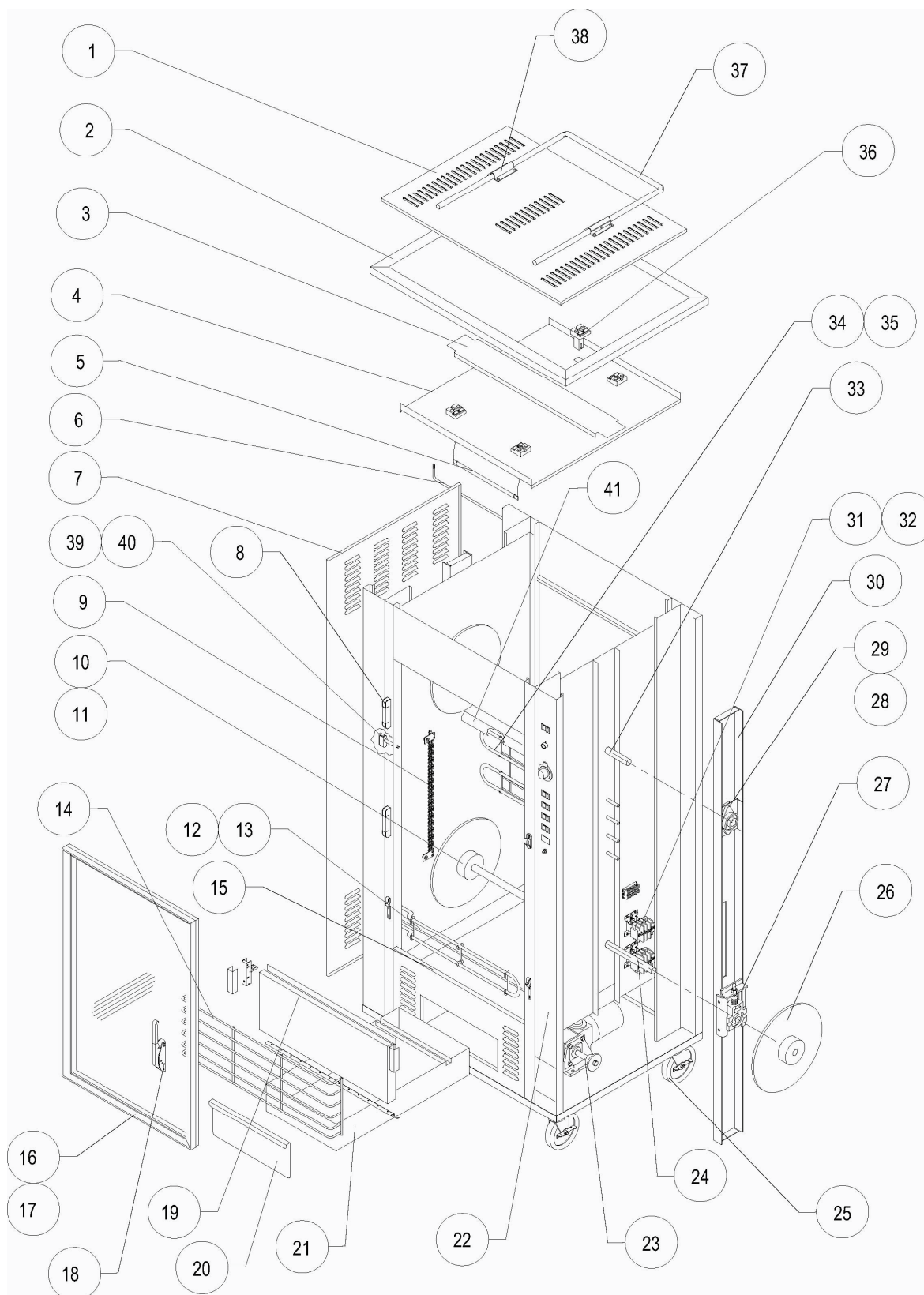
Figure 5. KS Oven
