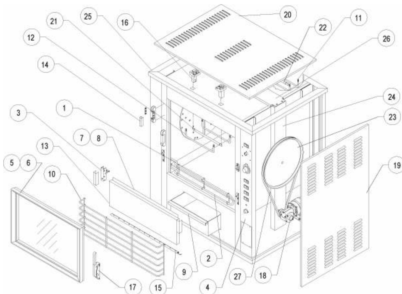
Figure 1. SR Oven
