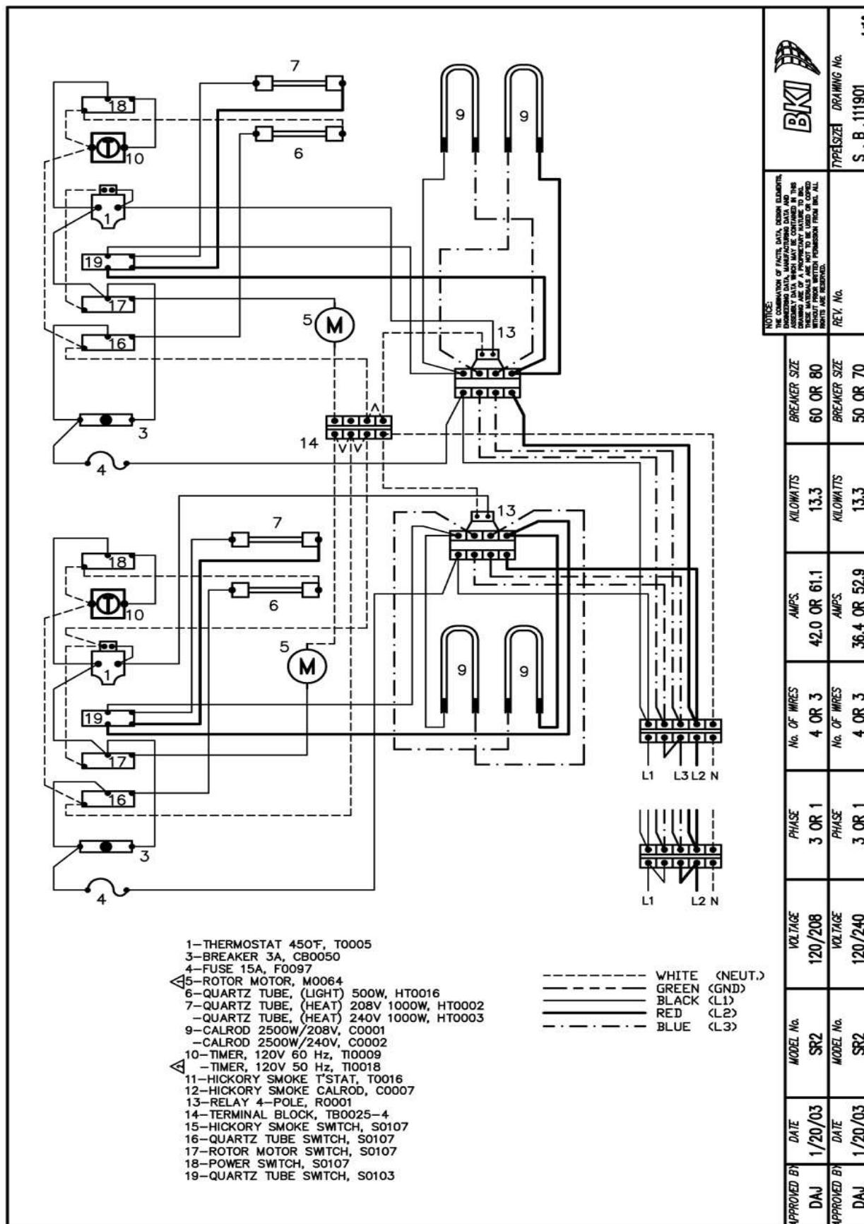
Figure 13. SR2 120V/208V and 120V/240V/1-3 Phase (Sheet 1 of 2)
