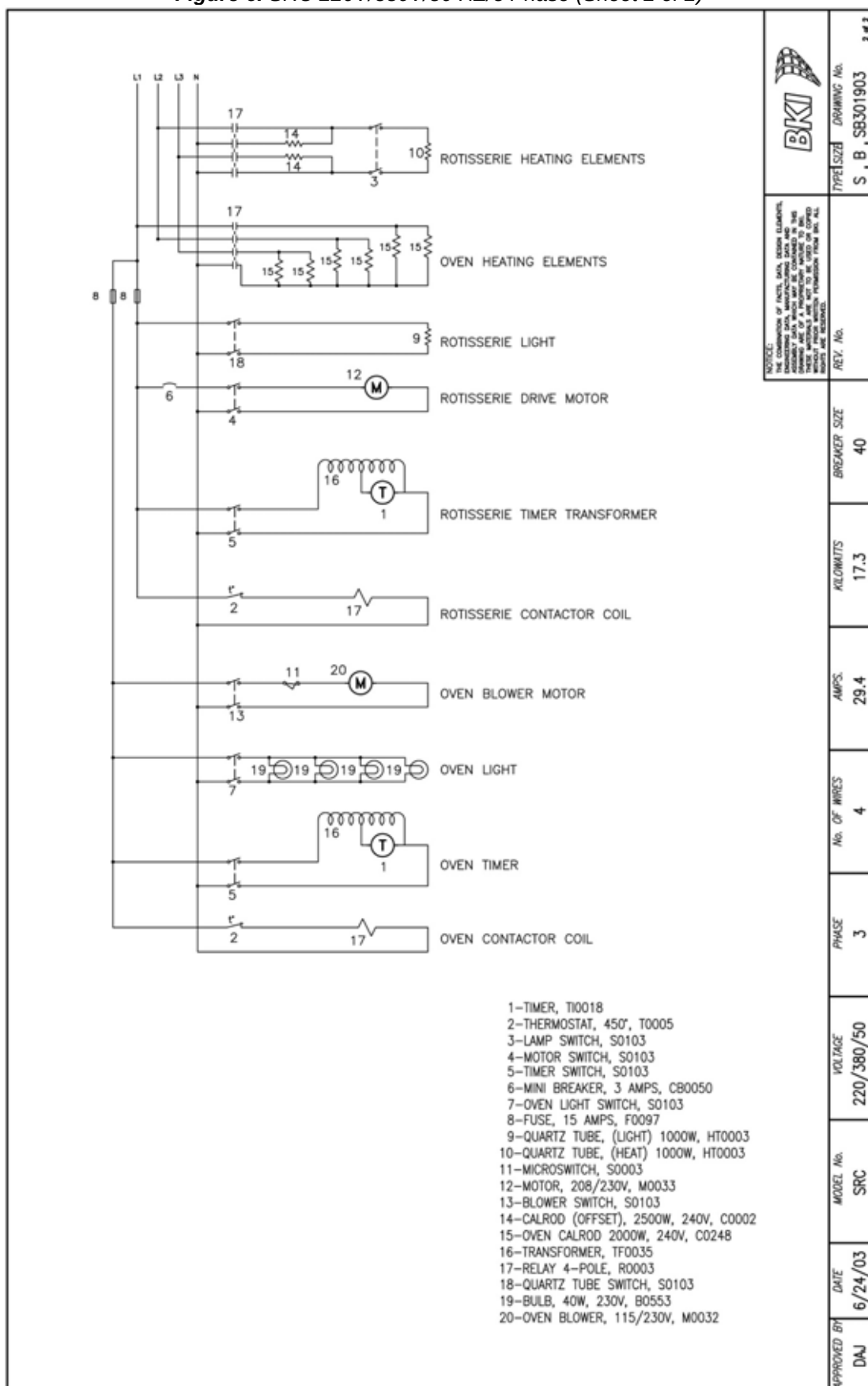
Figure 6. SRC 220V/380V/50 HZ/3 Phase (Sheet 2 of 2)
