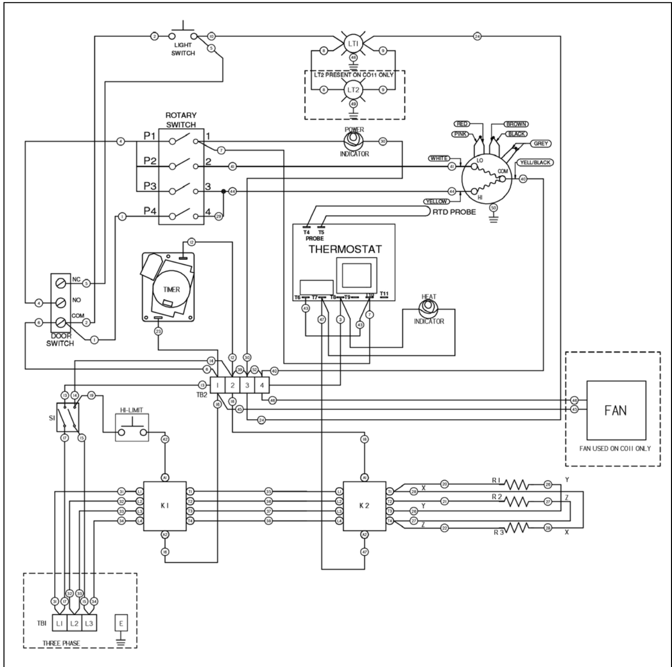
Wiring Diagram – C011-E COC-E 208/220/240V 3P
