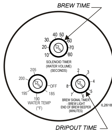
Fig. 15 Adjust BrewTime and Dripout Time
