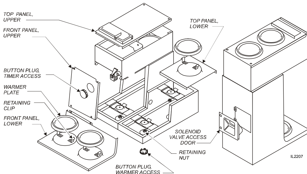
Fig. 13 Access Panels
