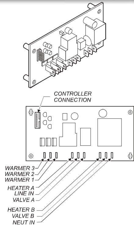
Fig. 19 Power Board Hook-Up
