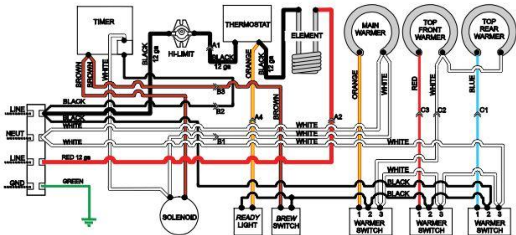
MODEL 9016 p/n 72358
