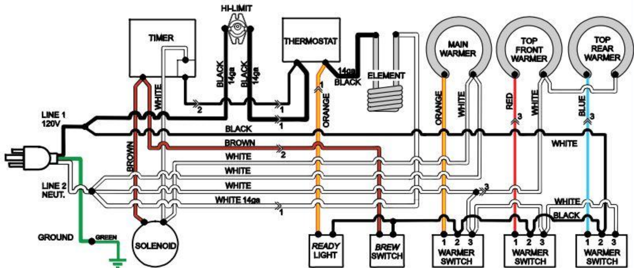
MODEL 9010 p/n 75446
