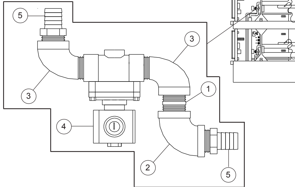
Steam Supply Assembly Bottom Section R8419
