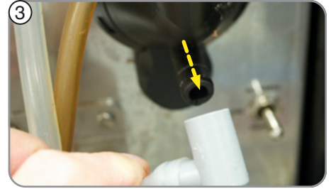
3. Remove the elbow fittings from both mixing chambers.
