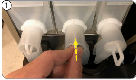
1. Push slide gates on the hopper elbows in to close.
