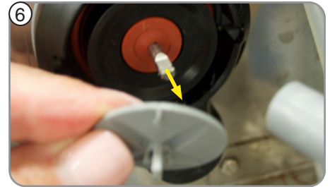
6. Remove frother disks (Impellers) from shafts by pulling straight out.
