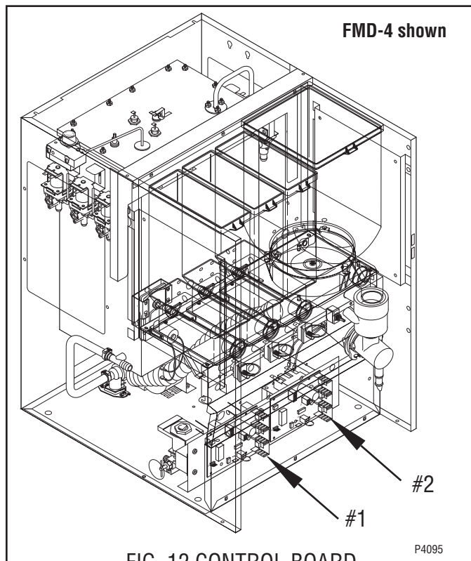
FIG. 12 CONTROL BOARD
