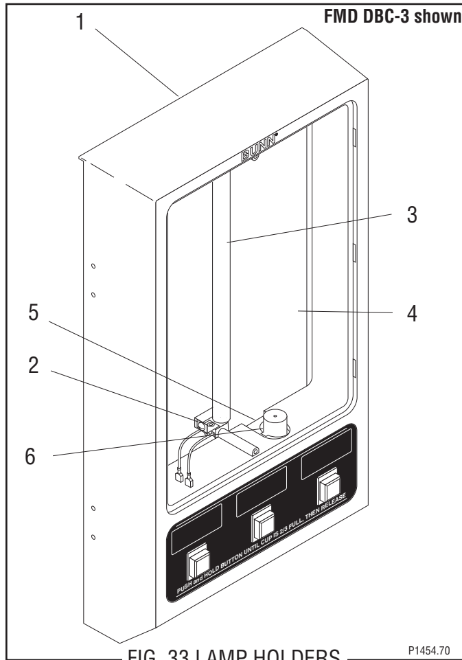
FIG. 33 LAMP HOLDERS
