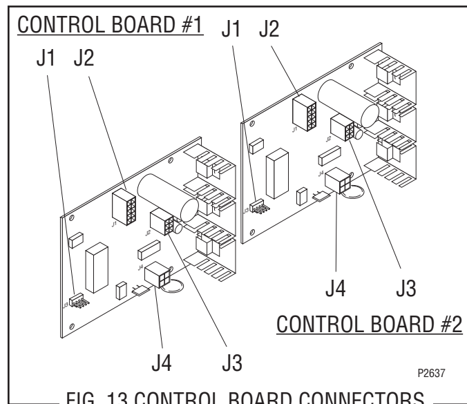
FIG. 13 CONTROL BOARD CONNECTORS
