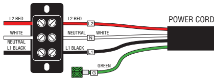
120/208-240V 3 WIRE + GROUND
