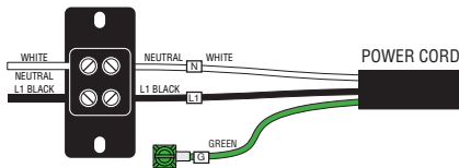
120V 2 WIRE + GROUND
