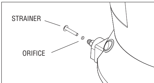
FIG. 3 Strainer and Orifice Location 120V
