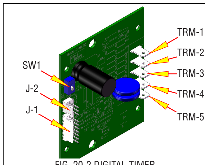
FIG. 20-2 DIGITAL TIMER
