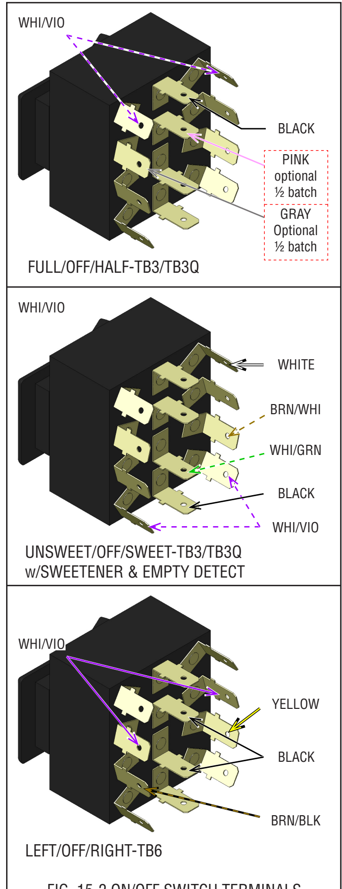
FIG. 15-2 ON/OFF SWITCH TERMINALS
