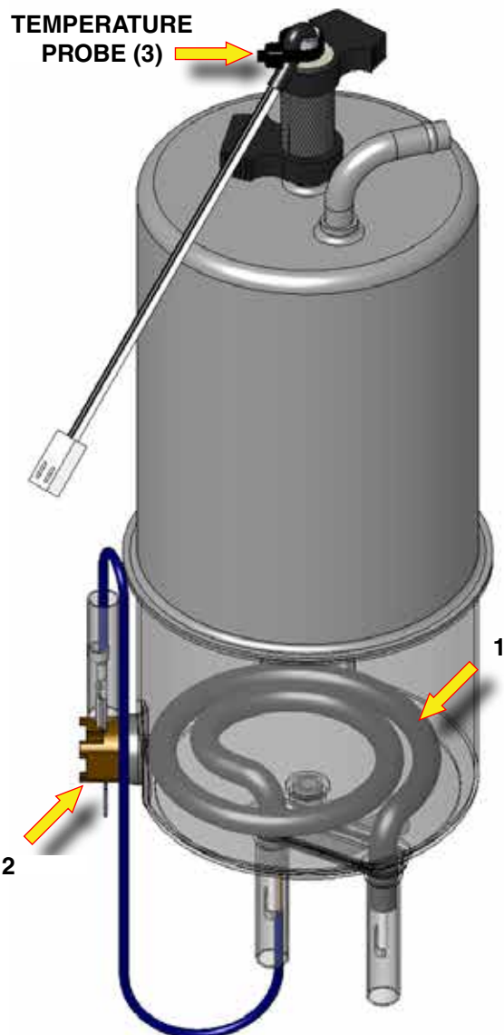
FIG. 16-1 TANK HEATER (1)
