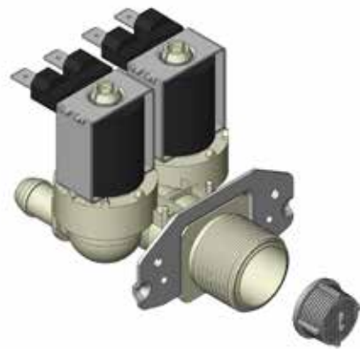
FIG. 14-2 EXPLODED VIEW
