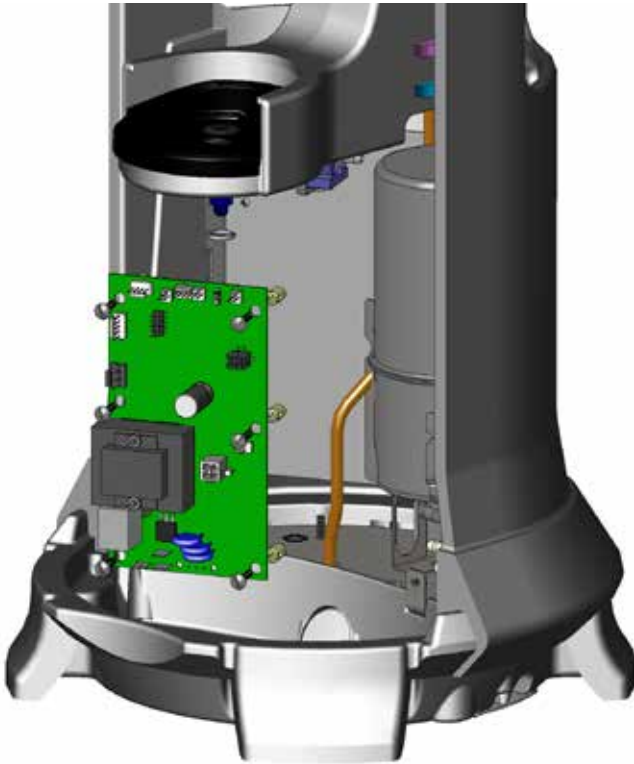
FIG. 11-1 CONTROL BOARD
