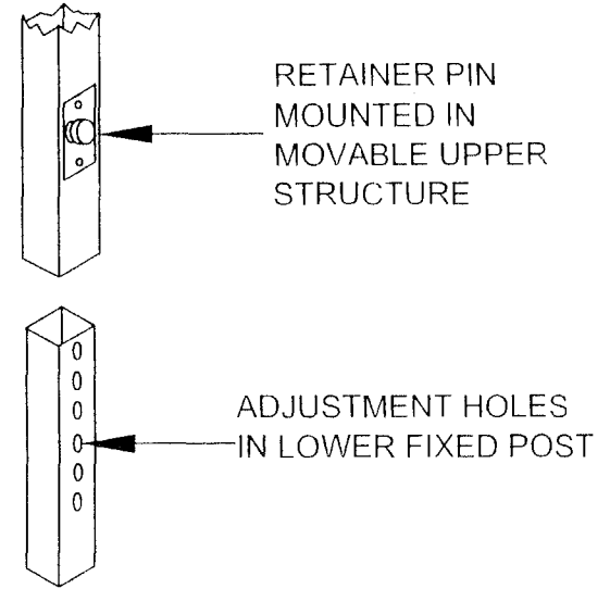
ADJUSTABLE LEG DETAIL
