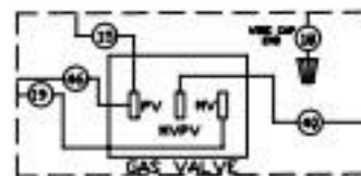
DETAIL A - HONEYWELL VALVE
