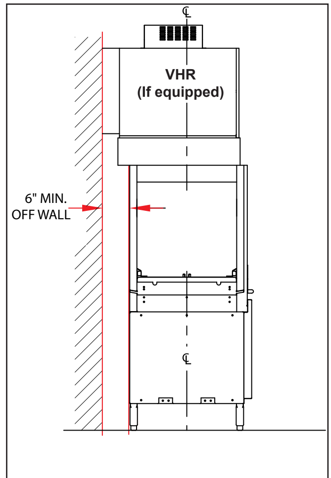
Fig. 2 - Nominal wall clearance for all machine models
