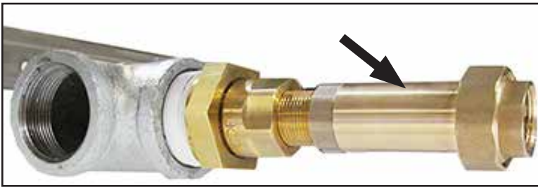
Fig.13 - Mechanical DWT shown installed in drain line.
