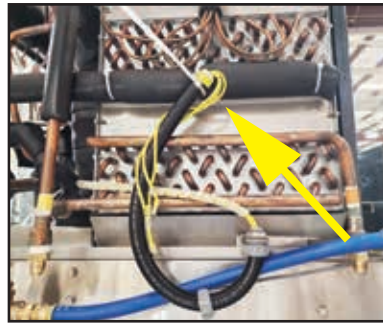
Detail Step 6: Install compressor cable bracket. Route cable to control cabinet.
