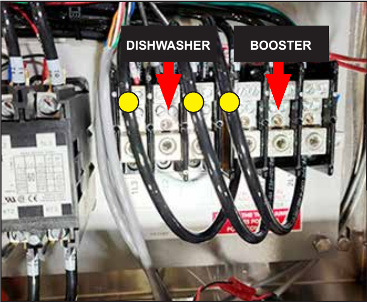
Fig. 25 - Jumpers installed for 1-point connection
