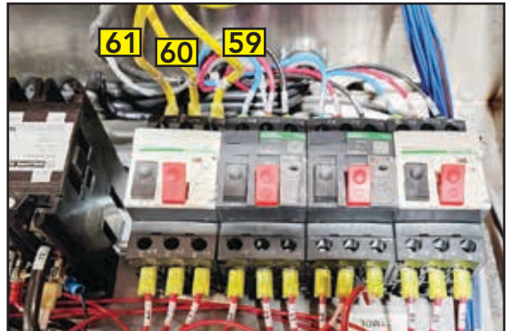
Detail Step 8: Connect compressor wires #59, #60 and #61 to 4MOL overload.
