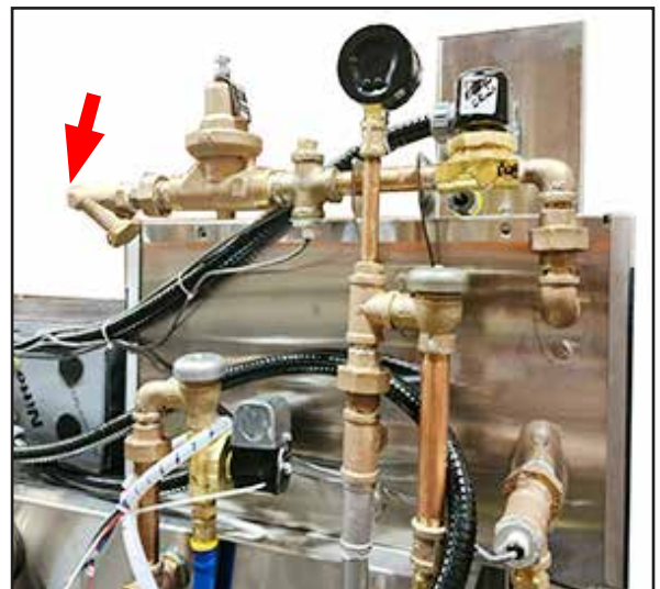
Fig. 12 - Heat recovery cold water connection
