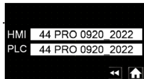
Fig. 34 - PLC software version number.
