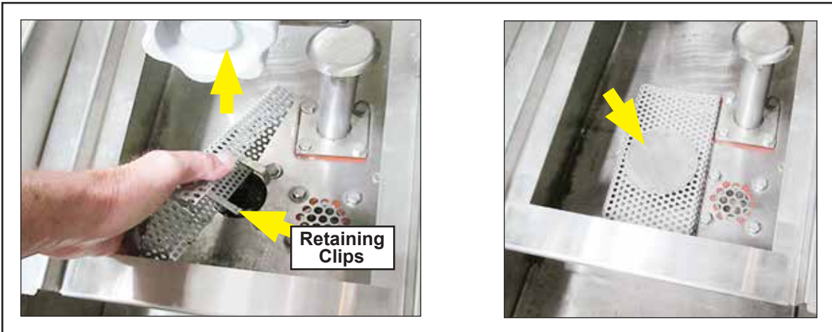
Fig. 83 - Front feed pump suction strainer
