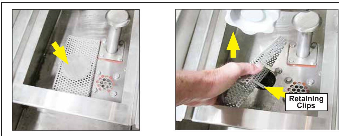
Fig. 70 - Prewash pump suction strainer
