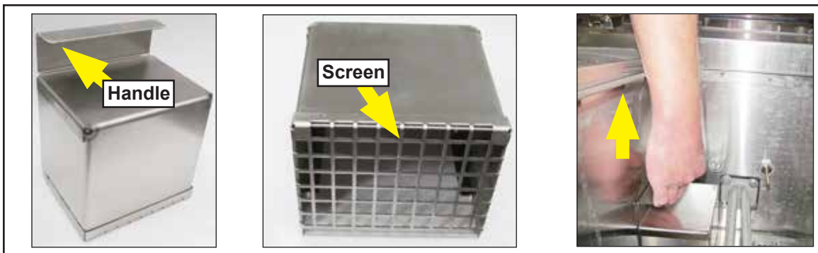
Fig. 69 - Wash tank pump suction strainer
