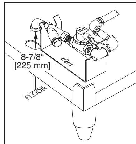
Figure 6 Hot Water Connection 3/4" NPT (D-H1T Only)
