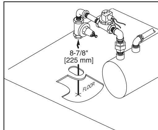
Figure 5 Hot Water Connection 3/4" NPT (D-HBT Only)
