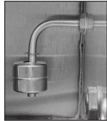
Figure 14 Float Switch
