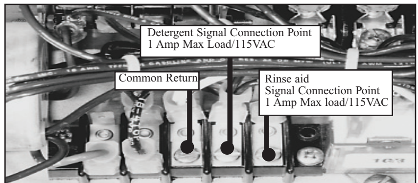
Figure 8 Chemical Signal Connection Points
