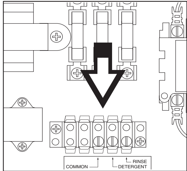
Figure 7 Chemical Dispenser Signal Terminal Block
