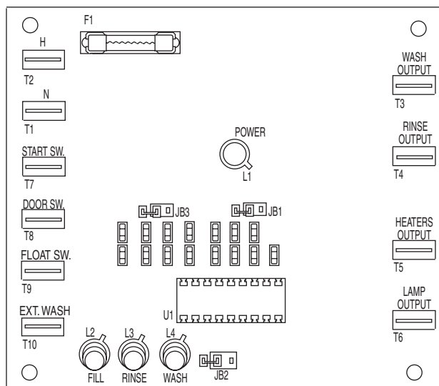
Figure 13 Solid State Control Board (112676 Shown)
