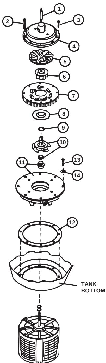
Figure 4 — Pump Assembly
