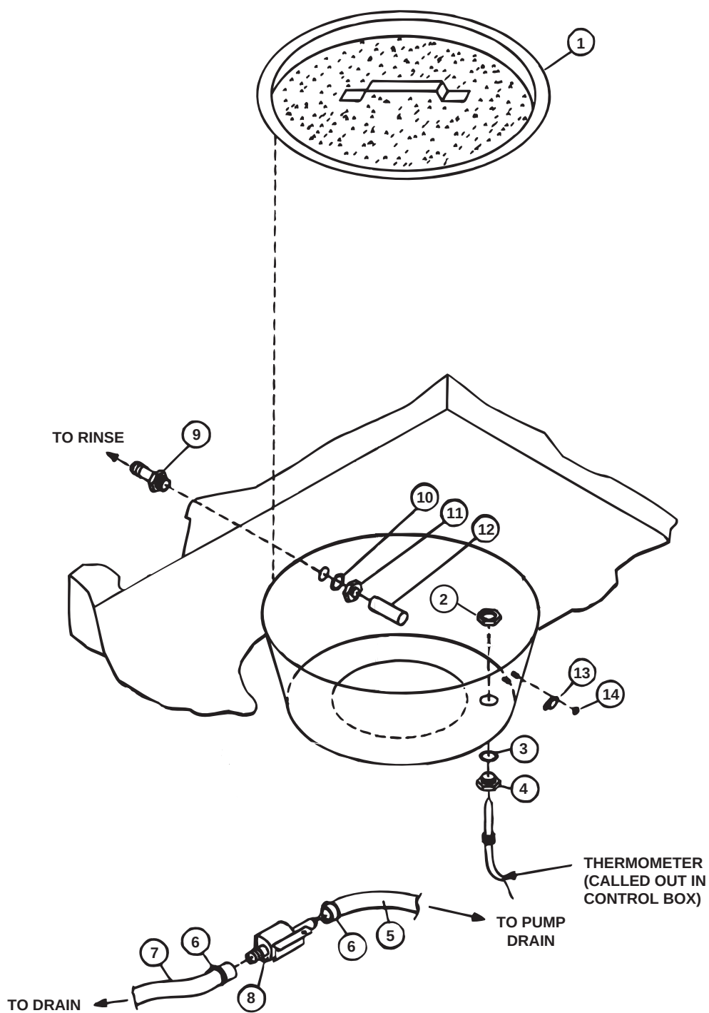
Figure 3 — Tank/Drain Assembly
