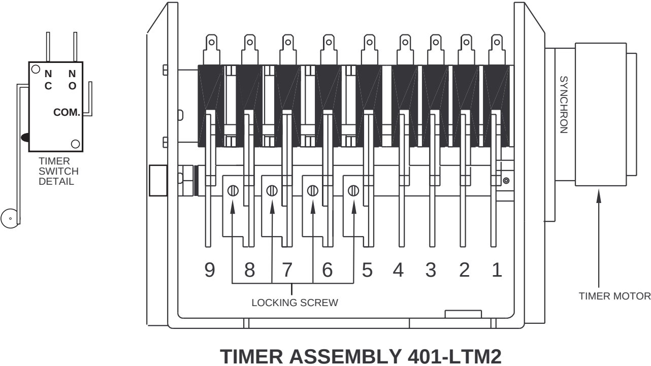
Figure 16 — Timer Chart and Diagram, 401-LT PLUS
