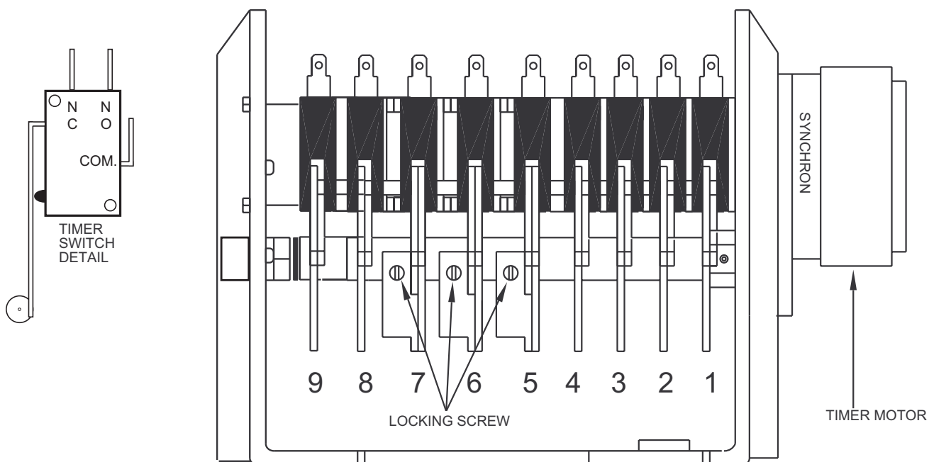
TIMER ASSEMBLY 401-HTM2
