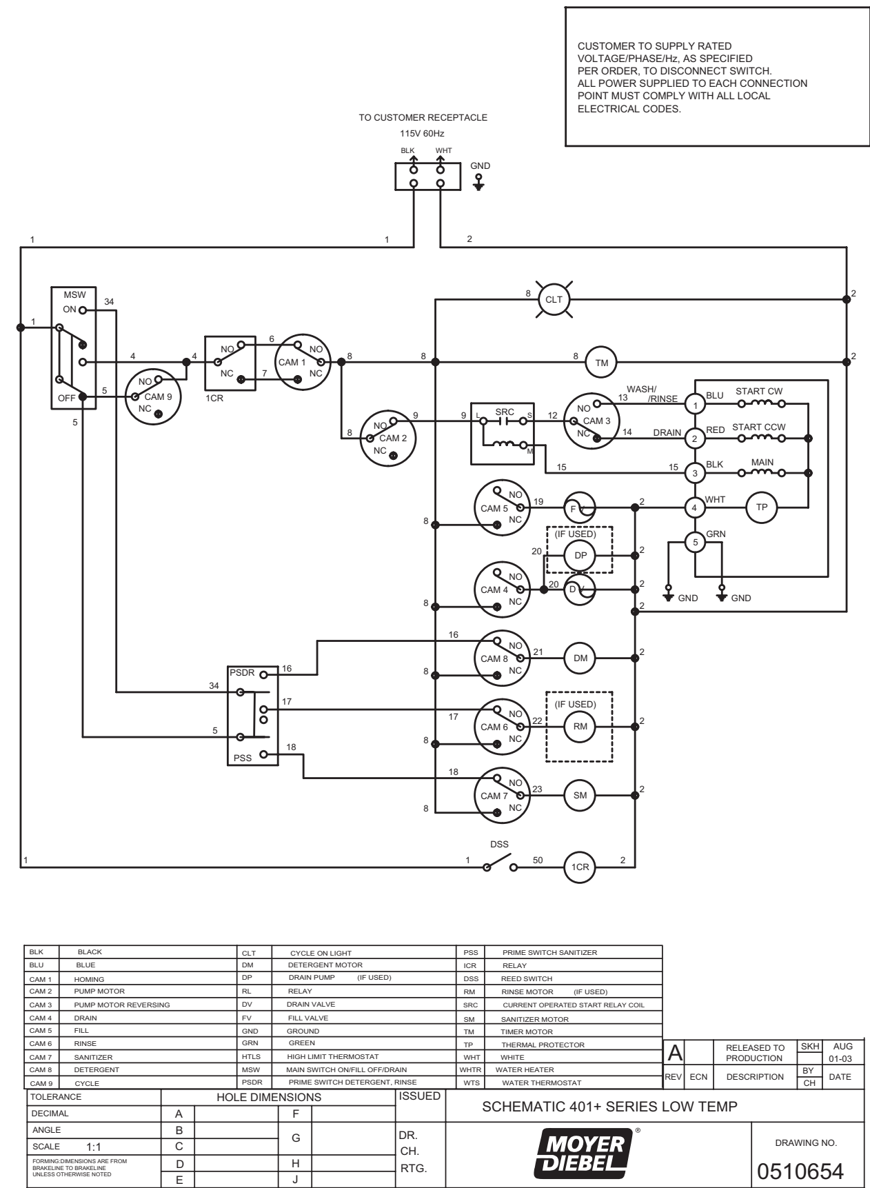
Figure 14 — Electrical Diagram, 401-LT PLUS
