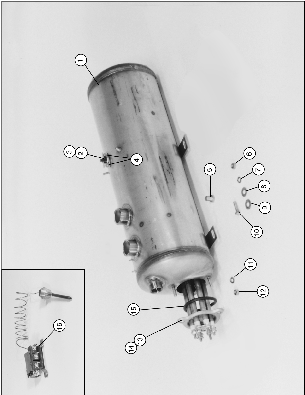
Figure 22 - Electric Booster Assembly and Thermostat
