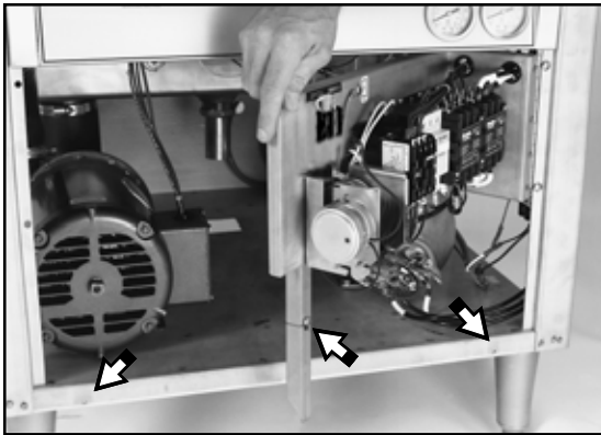
Figure 5 Hinged Control Panel Panel de control con bisagras
