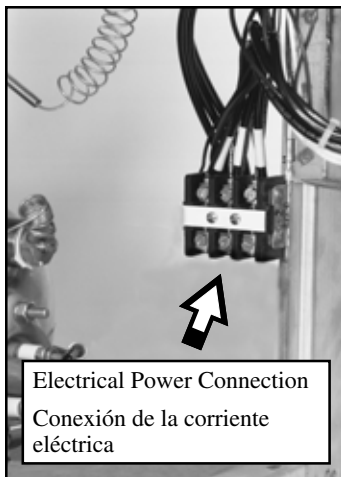
Figure 6 Main Terminal Block Bloque terminal eléctrico principal
