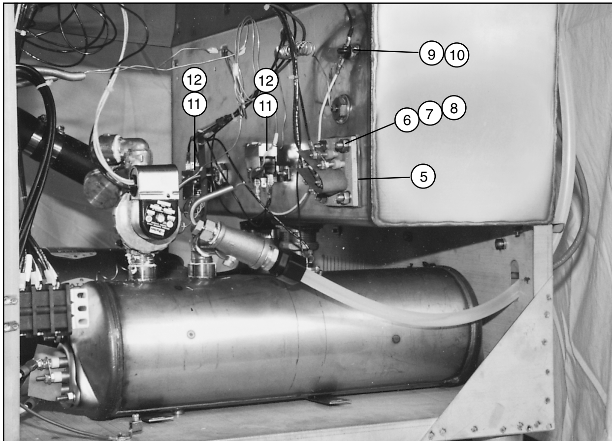
Figure 21 - Wash Tank Heater and Thermostats Calentador del tanque de lavado y termostatos
