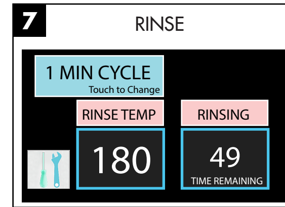
Monitor the final 'RINSE TEMP' to ensure it maintains a minimum of 180°F during the final rinse.
