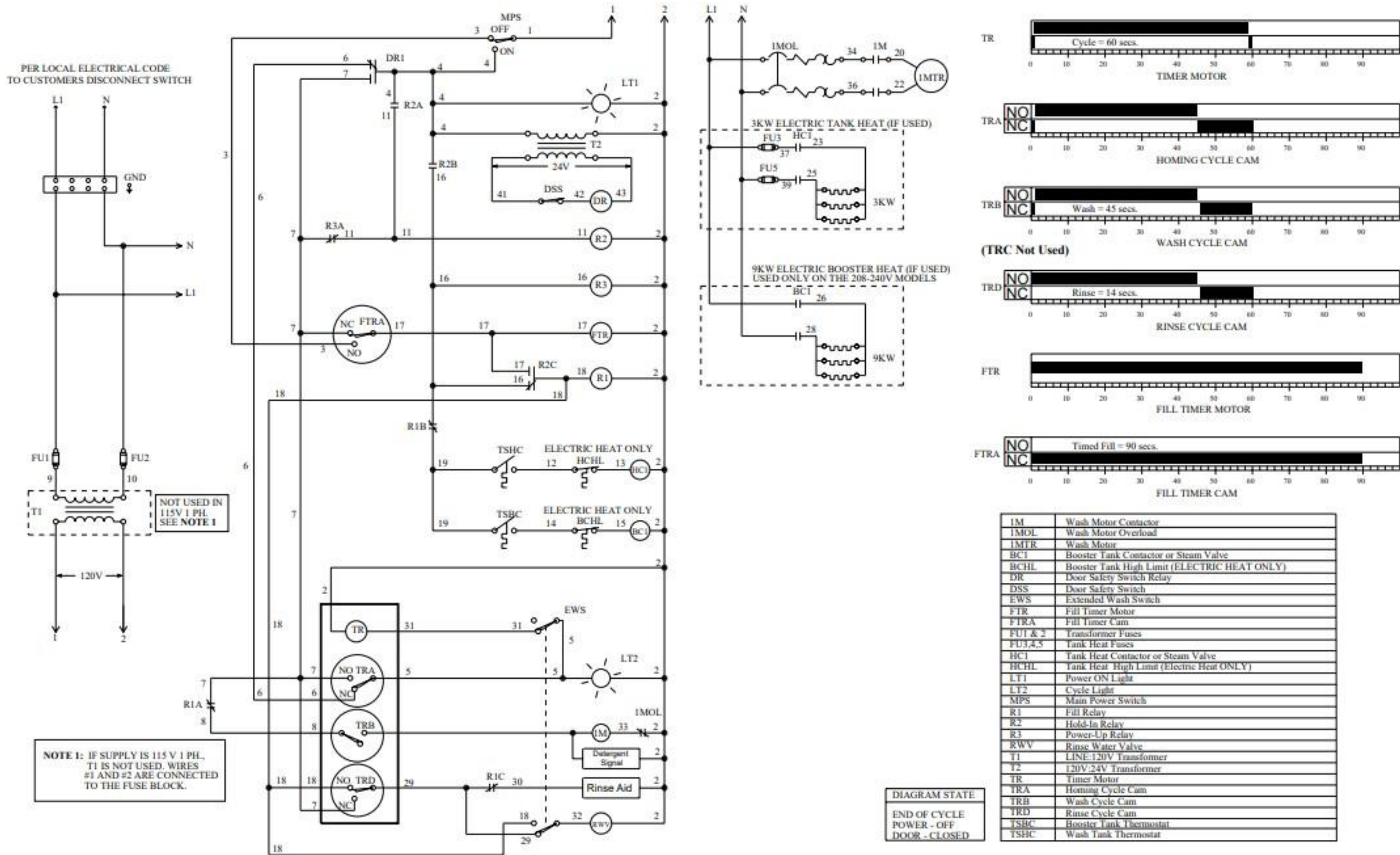
Figure 40 - Electrical Schematic / 1 Phase (MH-60, 6N, 6L)
