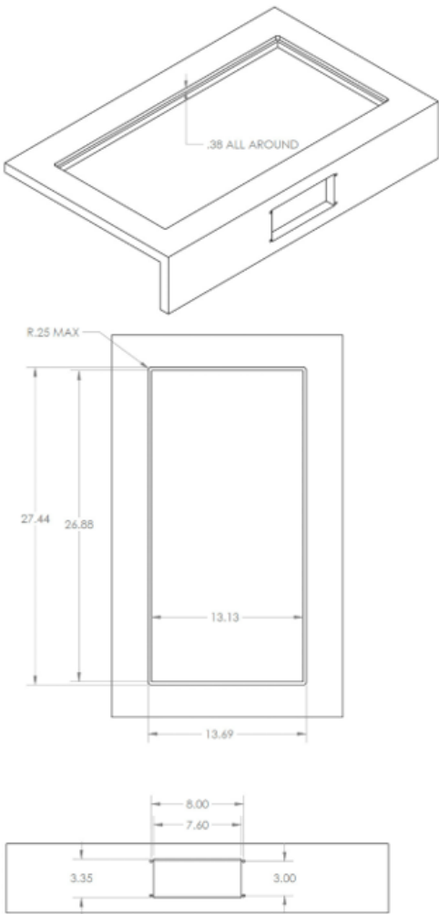
Flush Mount
