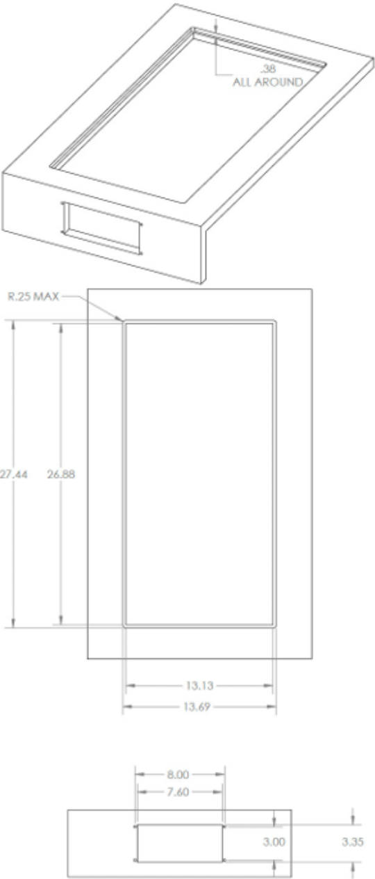
Flush Mount
