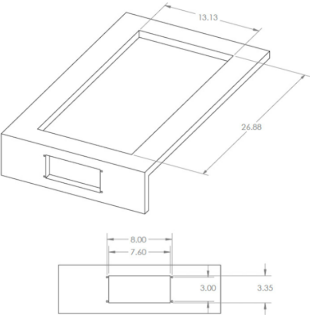
Top Mount
