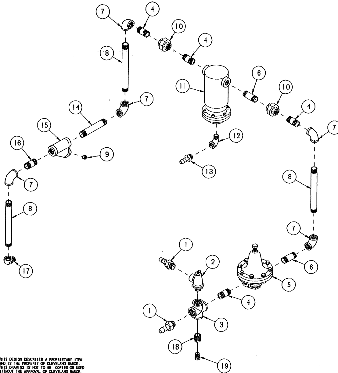
ASSEMBLED VIEW
