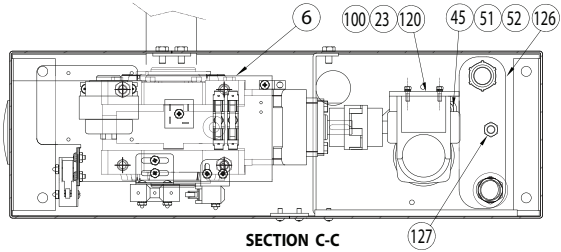
SECTION C-C
