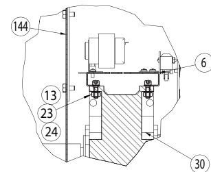
SECTION F-F
