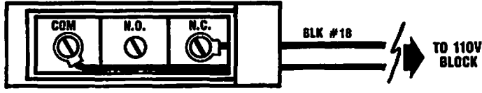
LIMIT SWITCH COVER PLATE REMOVED
