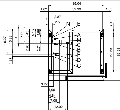
Connection points, unit floor
