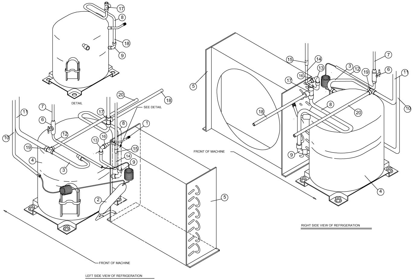
LEFT SIDE VIEW OF REFRIGERATION
