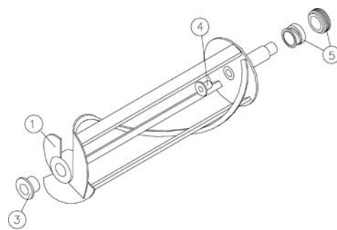
Figure W Dasher Assembly
