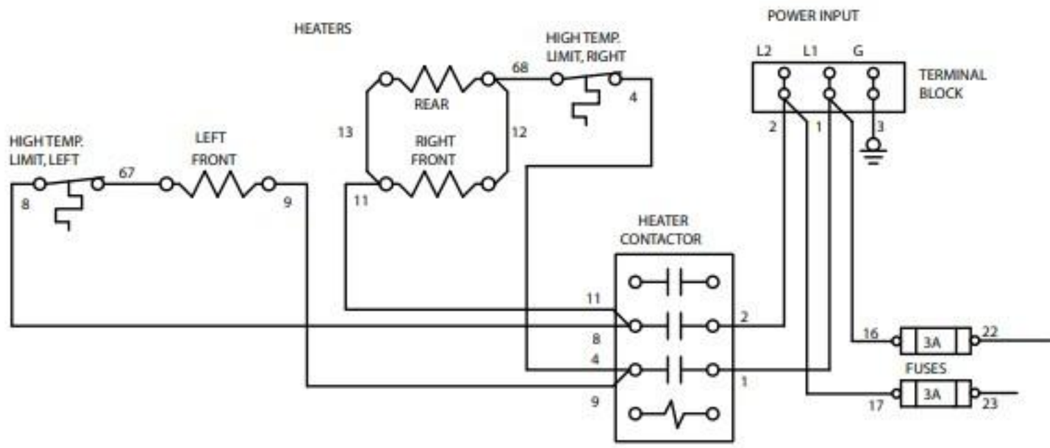
SINGLE PHASE WIRE KIT 5812-907
