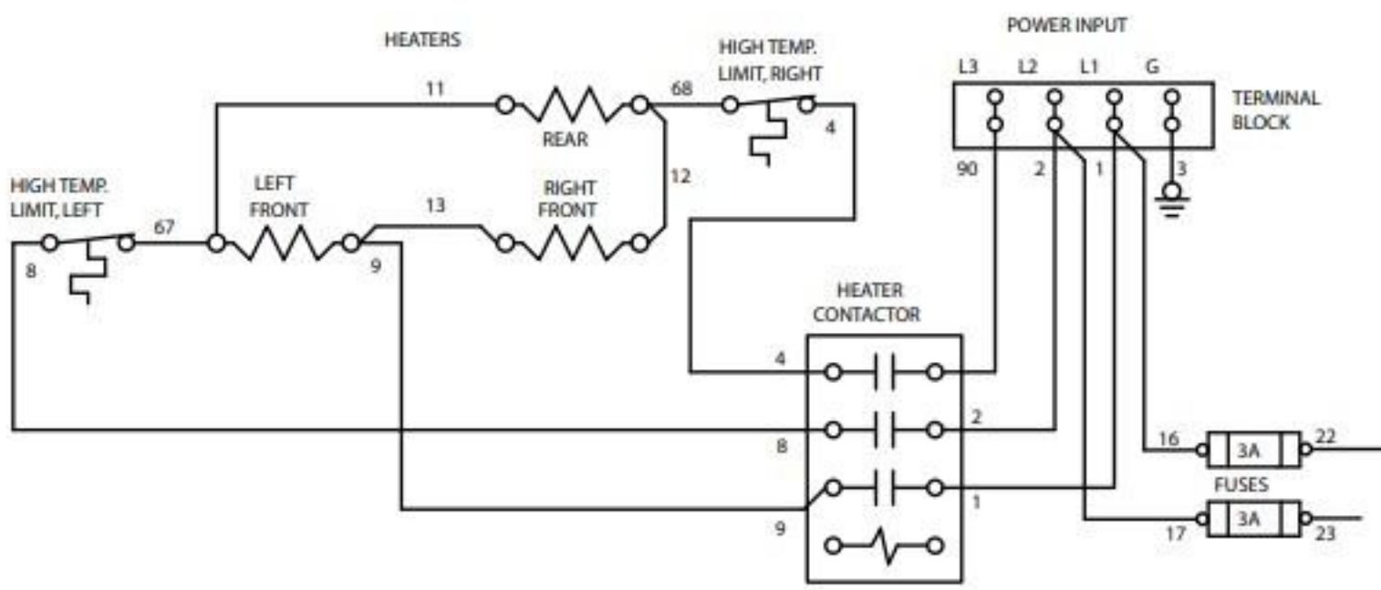
3 PHASE WIRE KIT 5812-908
