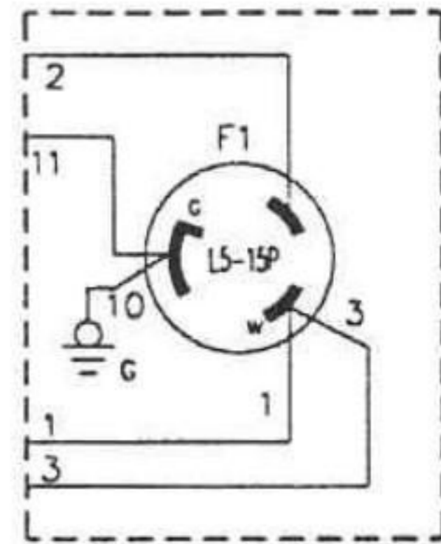
PLUG WIRING 120 VOLTS ONLY
