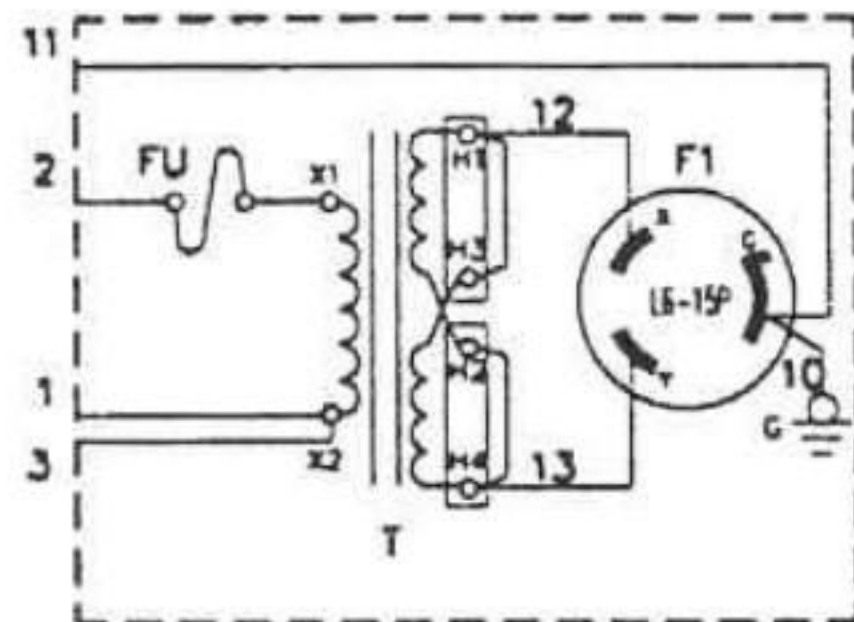
PLUG WIRING 240 VOLTS ONLY
