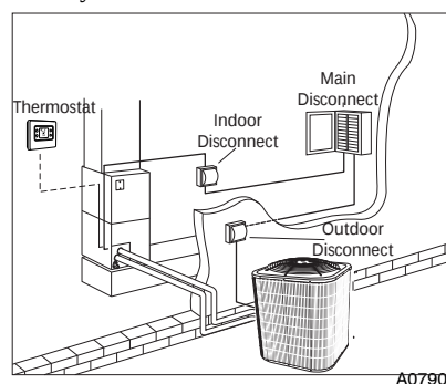
Fig. 1 - Electrical Disconnects
