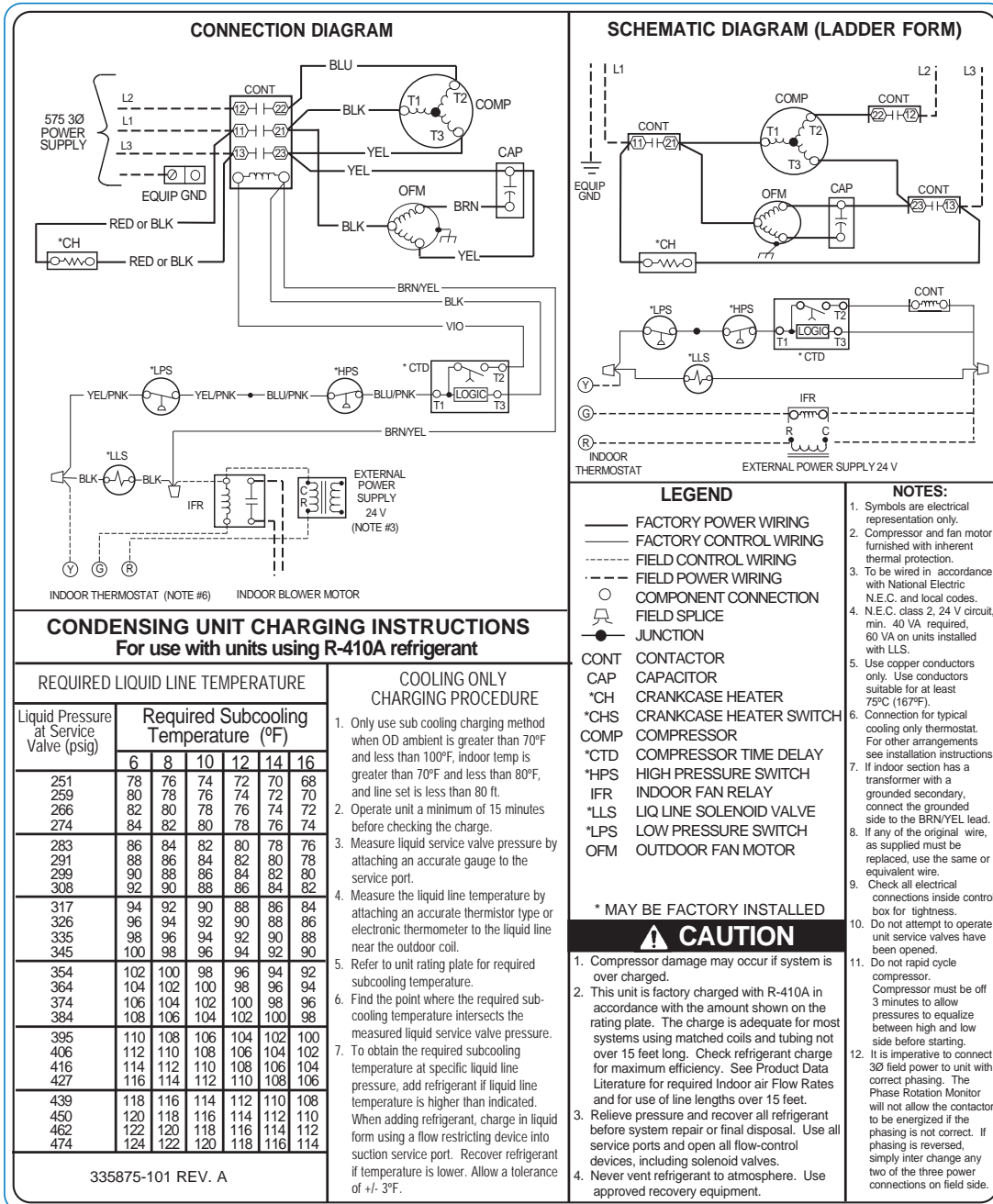
Fig. 3 – Wiring Diagram — Model size 3 - 5 tons, 575/3
