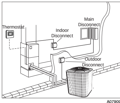
Fig. 1 - Electrical Disconnects
