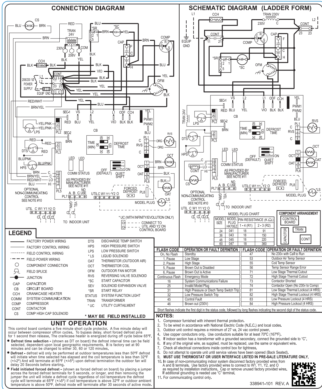
Fig. 1 – Wiring Diagram — Model size 2 - 5 tons, 208/230-1
