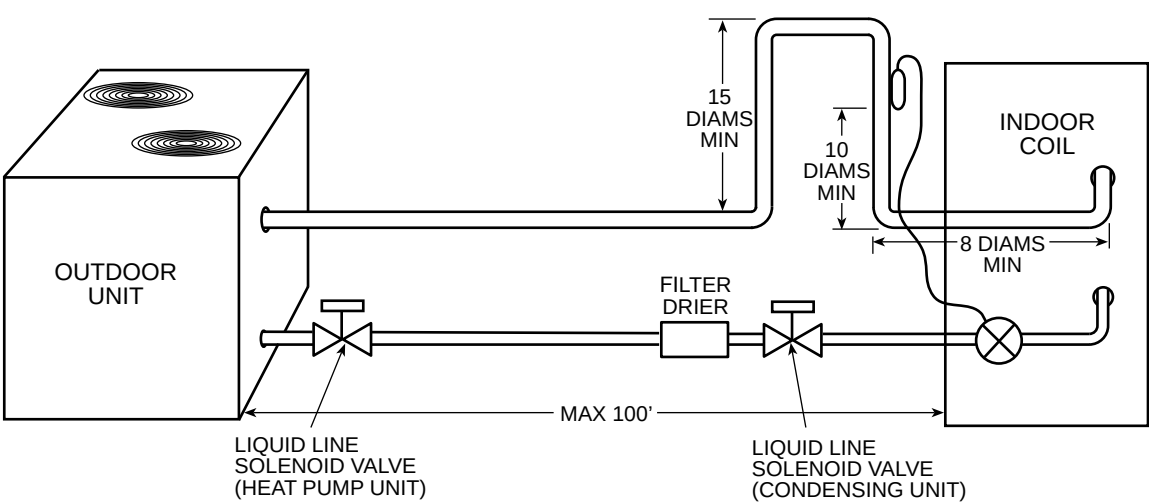
Typical Piping for Units on the Same Level
