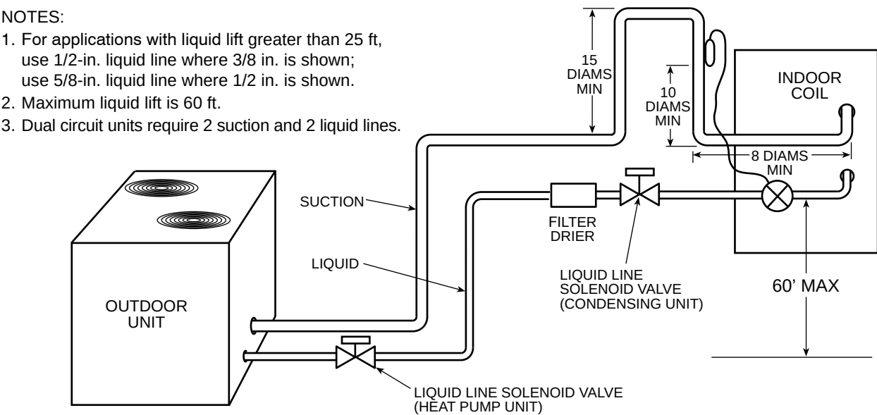
Typical Piping When Indoor Unit is Above the Outdoor Unit
